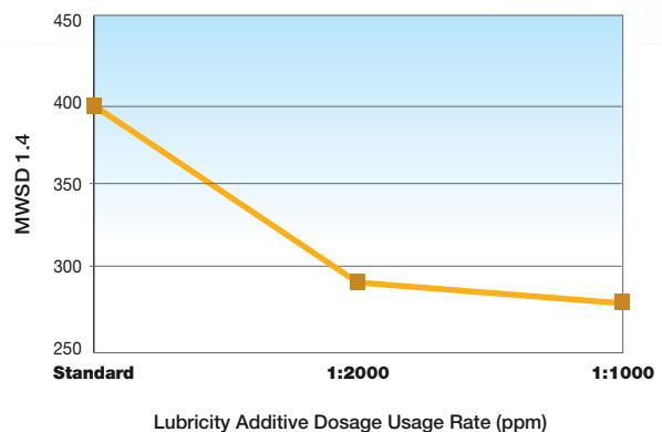
AR6400-D MAX - Friction Test Results
