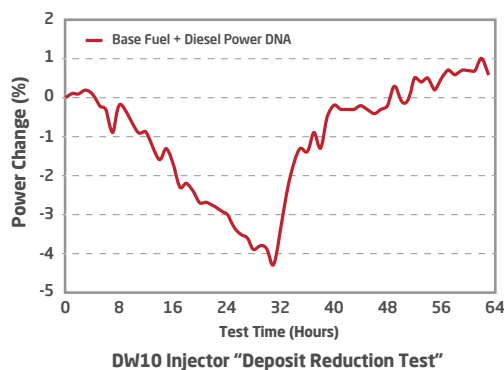
Engine Clean-Up Test
